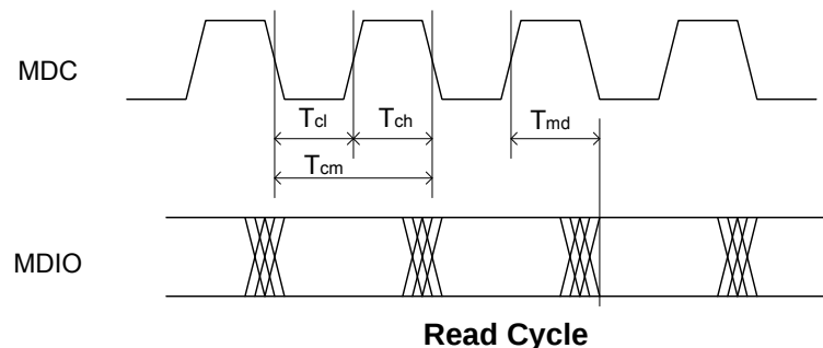
Figure 23 SMI Timing Requirements
