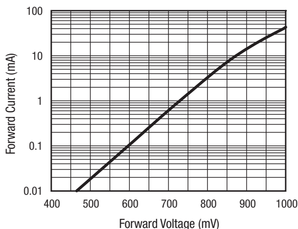
Figure 4. DC Characteristic
