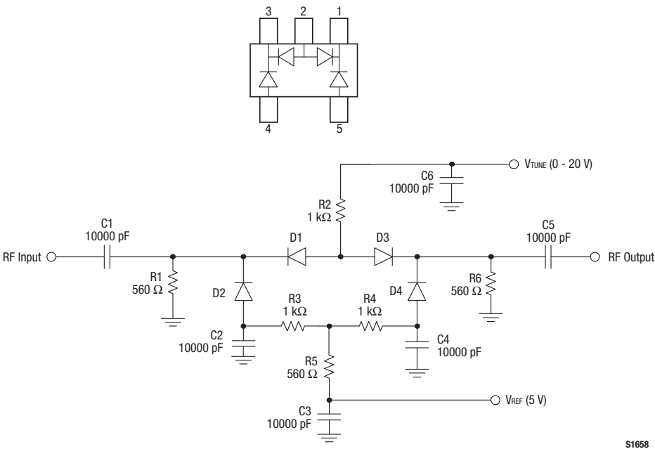
Figure 1. SMP1307-027 Block Diagram and Schematic
