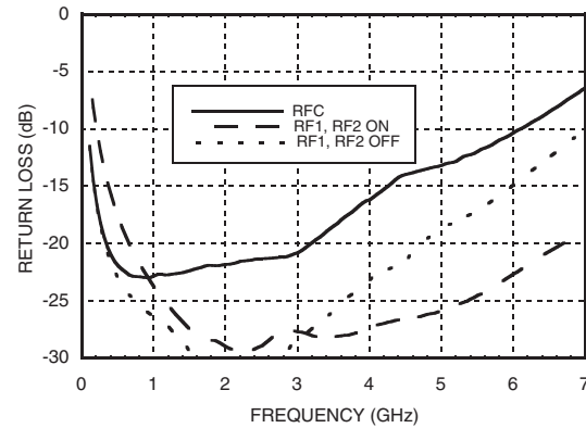
Return Loss [1]
