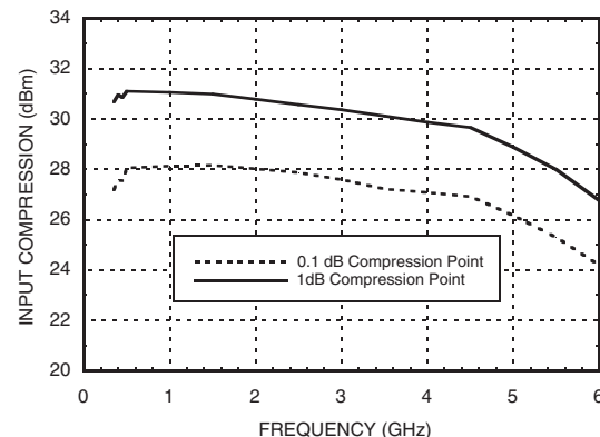
0.1 and 1 dB Input Compression Point, V dd = 3V
