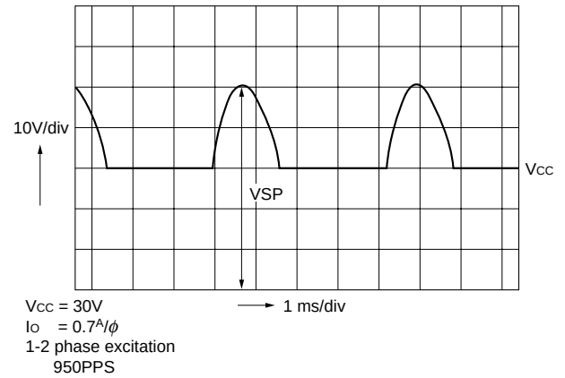
Example V_{SP} waveform
