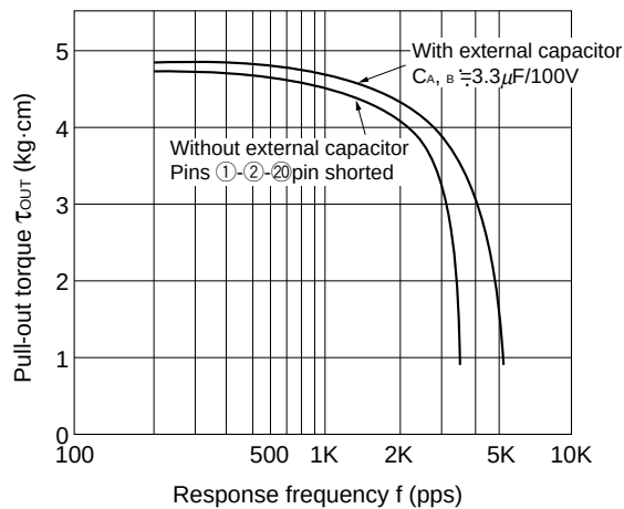
Torque vs. Response frequency
