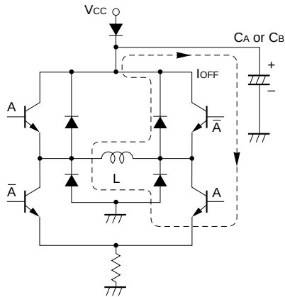
Charging path of the counter EMF
