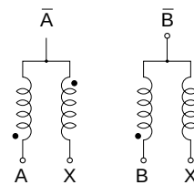
Motor connection
