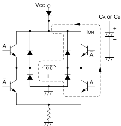
Discharge path of the counter EMF
