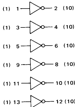
MC681 Hex Inverter (open collector) MC697 Hex Inverter (passive pull-up)
