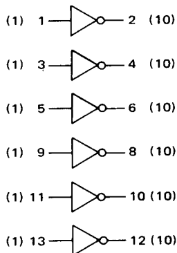
MC689 Hex Inverter (high voltage)
