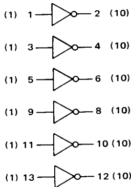
MC680 Hex Inverter (active pullup)
