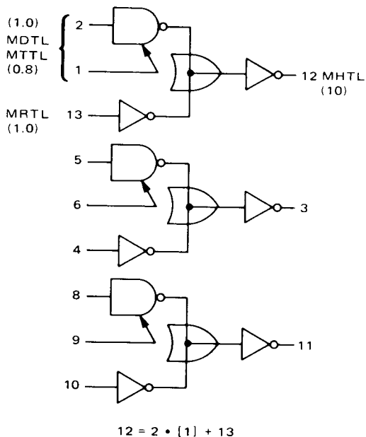
MC666 Triple Level Translator
