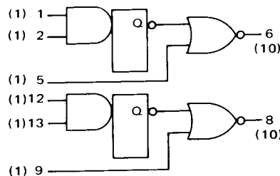
MC675 Dual Pulse Stretcher/Multivibrator
