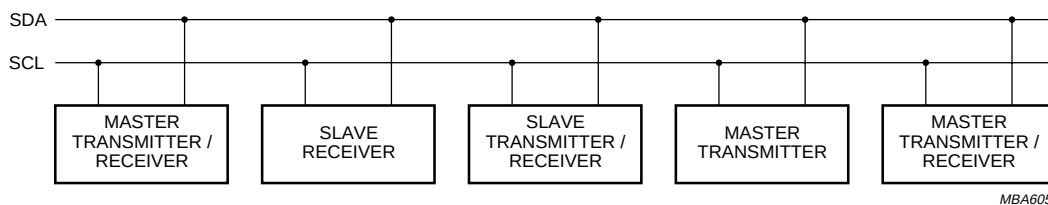
Fig 8. System configuration.
