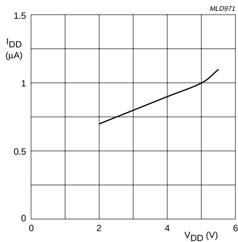
Fig 16. I_{DD} as a function of V_{DD} ; CLKOUT = 32 kHz.
