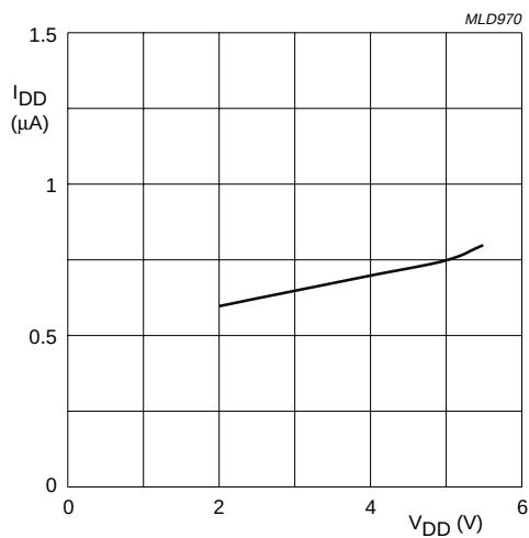
Fig 15. I_{DD} as a function of V_{DD} ; CLKOUT disabled.
