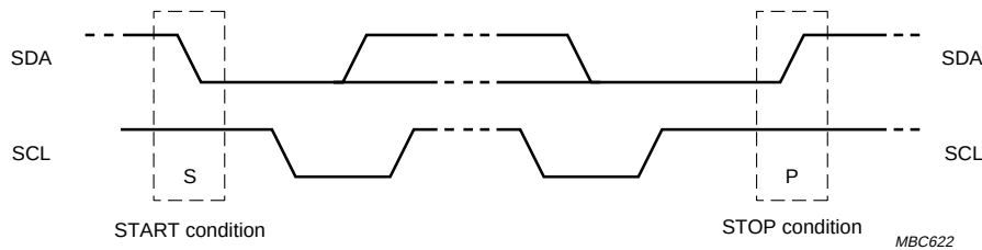
Fig 7. Definition of start and stop conditions.
