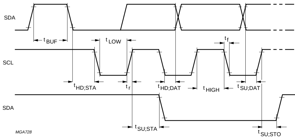
Fig 14. I 2 C-bus timing waveforms.
