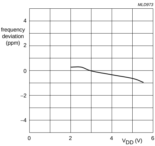
Fig 18. Frequency deviation as a function of V_{DD} .
