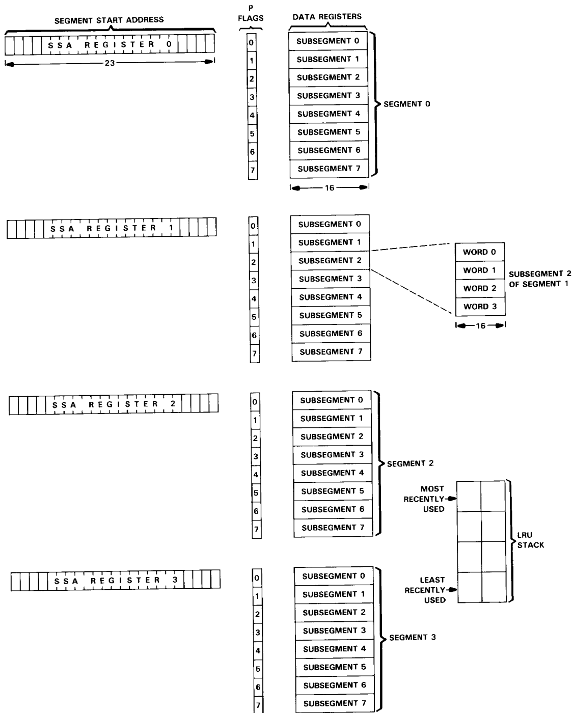
FIGURE 3. INSTRUCTION CACHE
