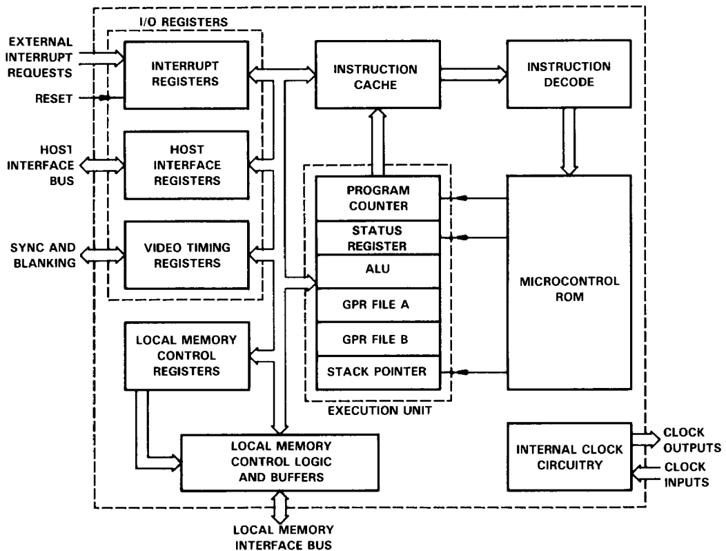
FIGURE 1. TMS34010 INTERNAL ARCHITECTURE
