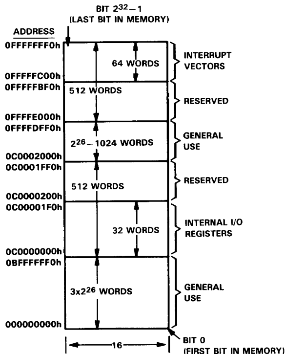
FIGURE 6. MEMORY MAP
