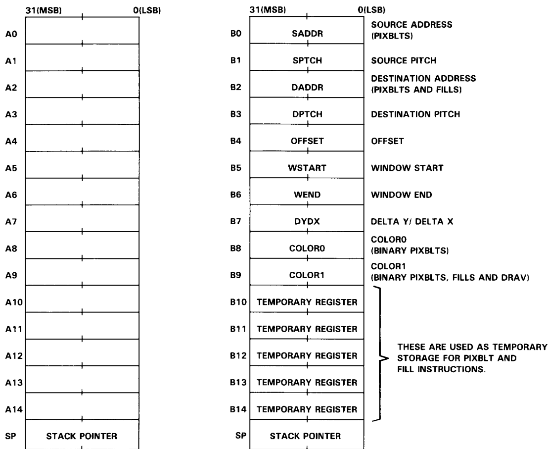
FIGURE 2. REGISTER FILES A AND B
