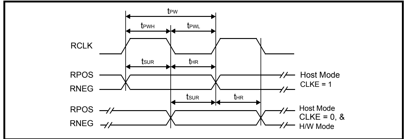
Figure 8: LXT305A Receive Clock Timing Diagram
