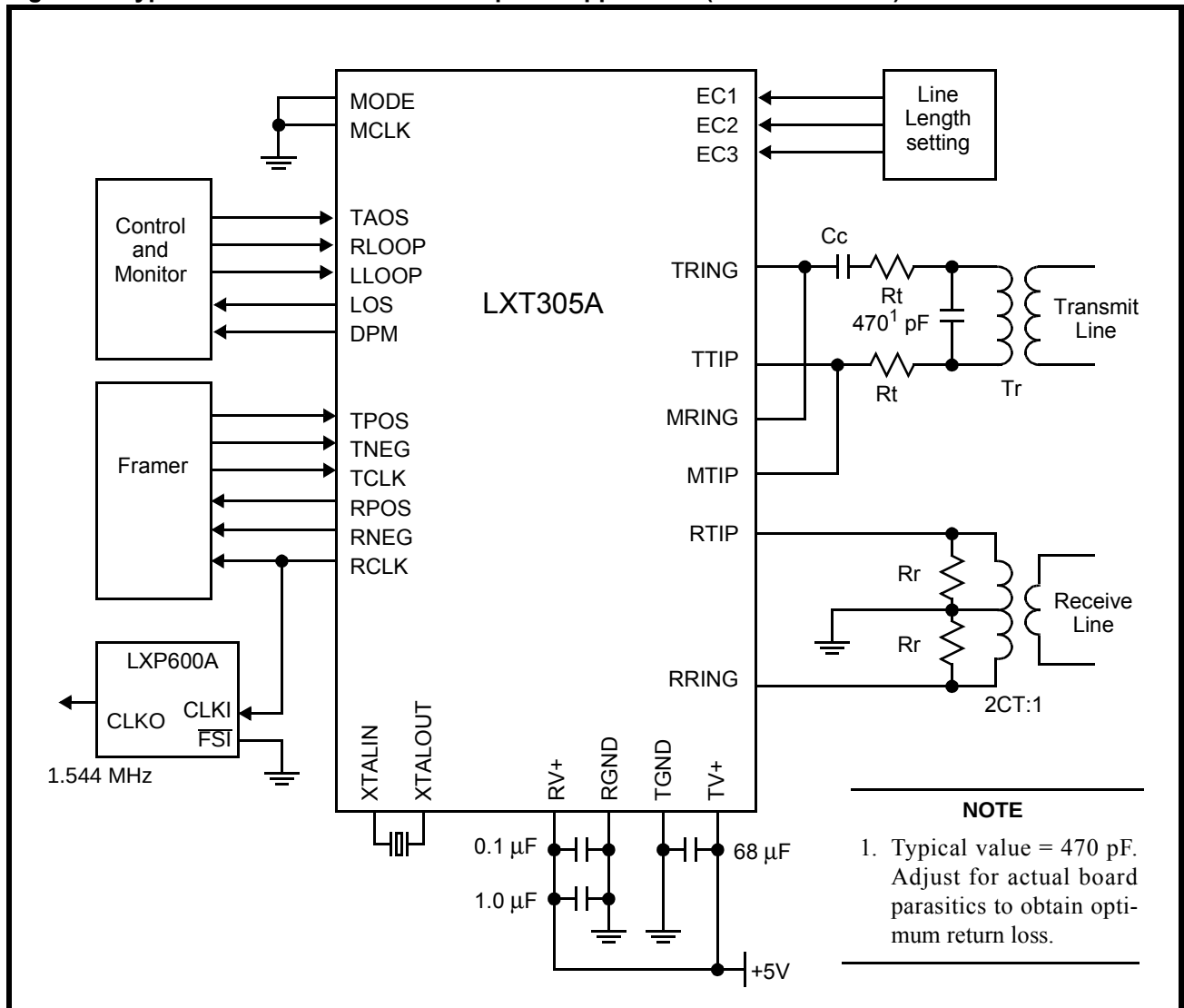
Figure 5: Typical LXT305A 120 \Omega 2.048 Mbps E1 Application (Hardware Mode)
