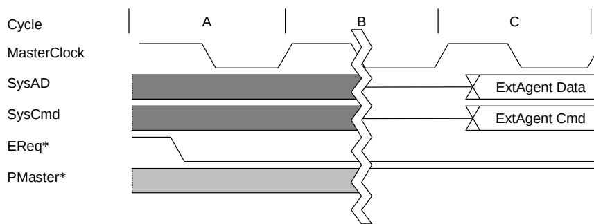
Figure 11.3.10 Sample Cycle with EReq* Asserted
