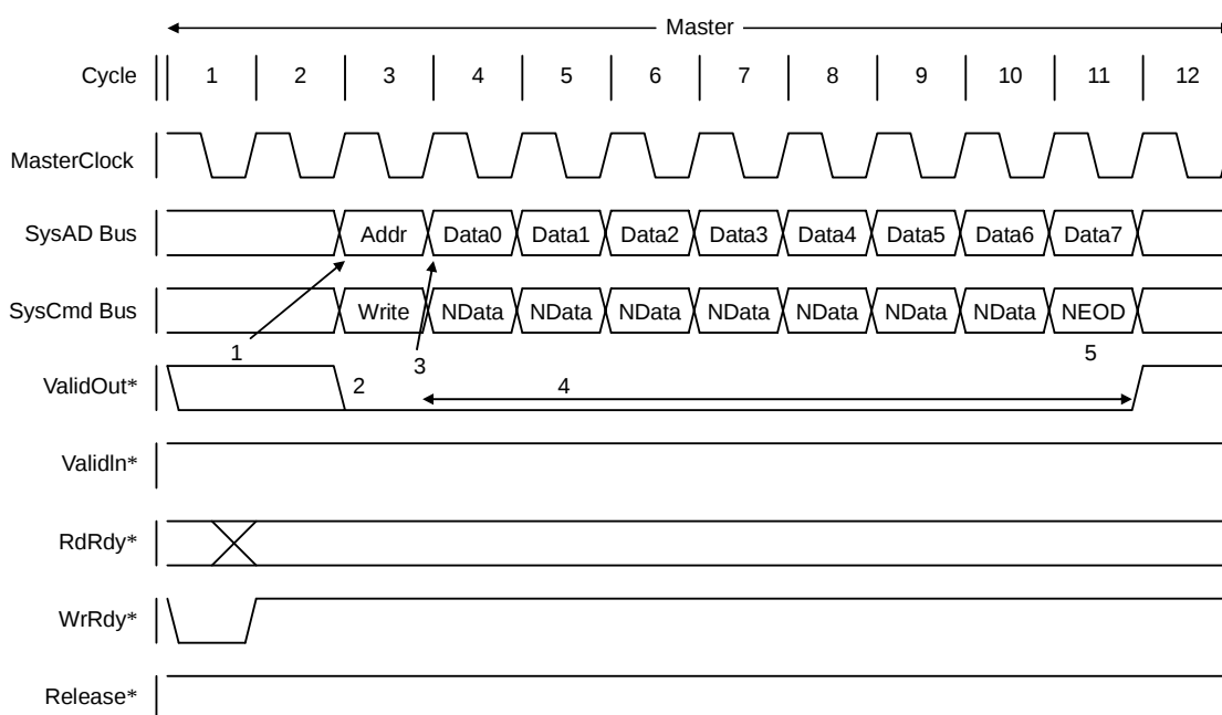
Figure 11.2.17 Processor non-coherent block request protocol
