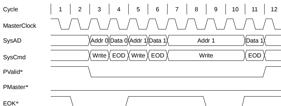
Figure 11.3.15 Processor Single Write Request Followed By A Cancelled And Retried Write Request
