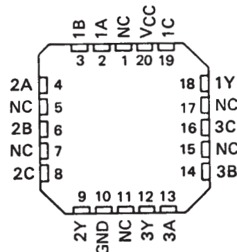
SN54LS15, SN54S15 . . . FK PACKAGE
