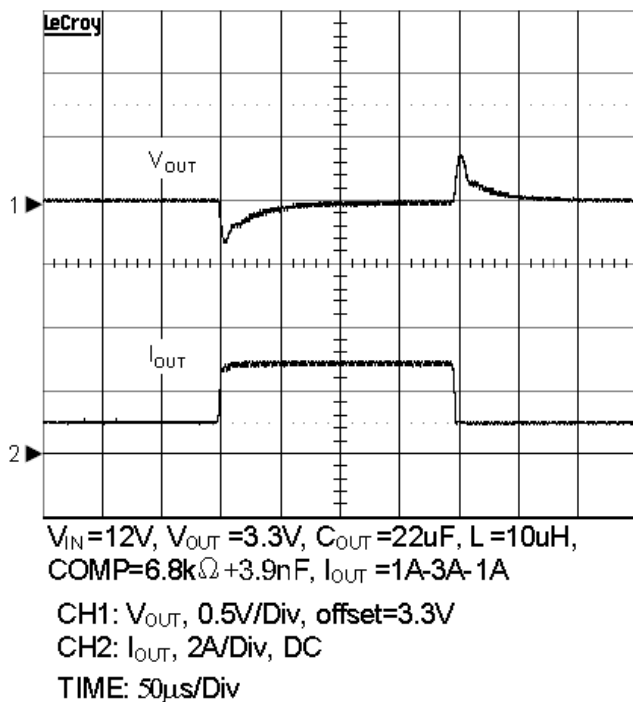
Load Transient
