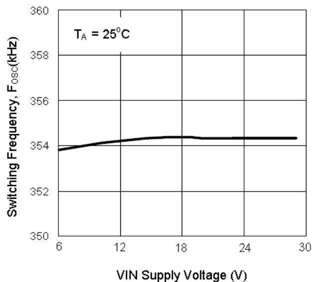
Switching Frequency vs. VIN Supply Voltage
