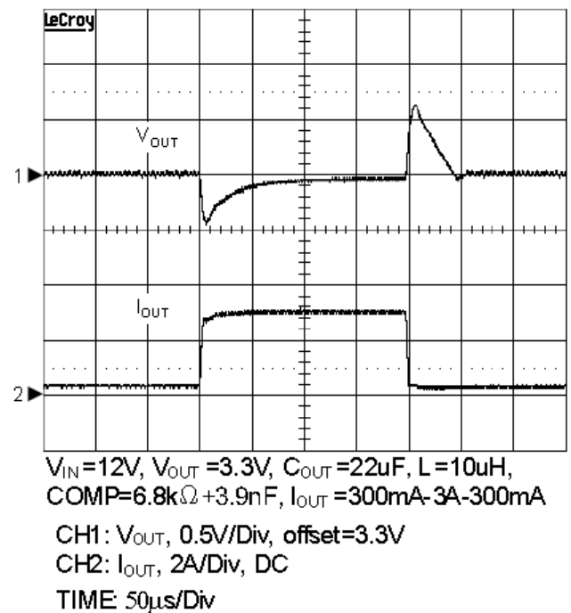
Load Transient
