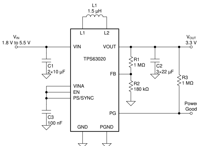
Simplified Schematic
