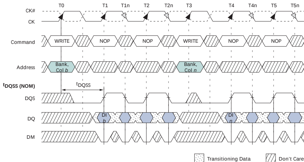
Figure 40: Nonconsecutive WRITE-to-WRITE
