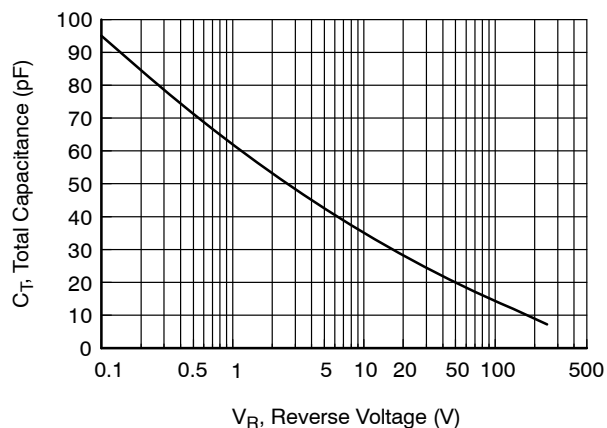
Figure 3. Total Capacitance
