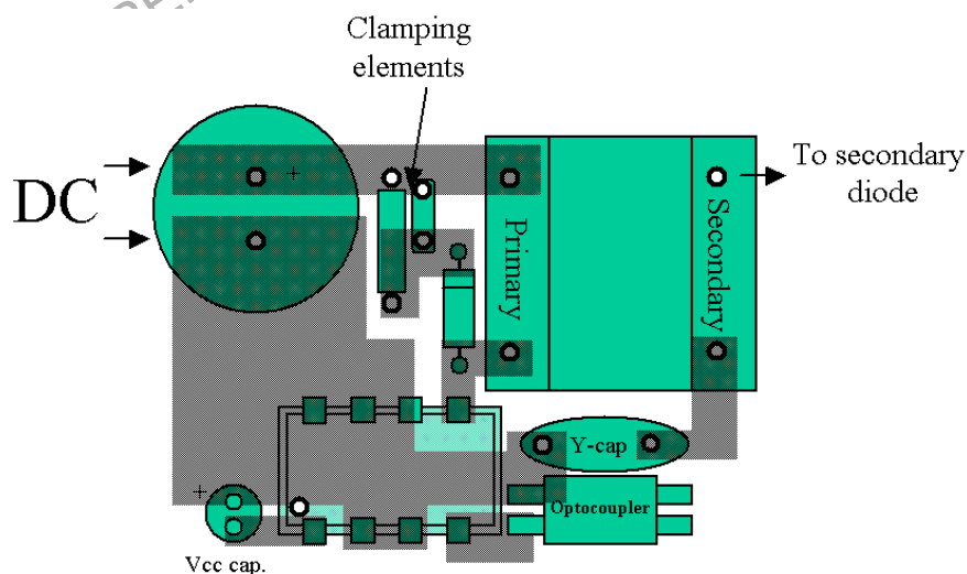
Figure 27. A Possible PCB Arrangement to Reduce the Thermal Resistance Junction-to-Ambient
