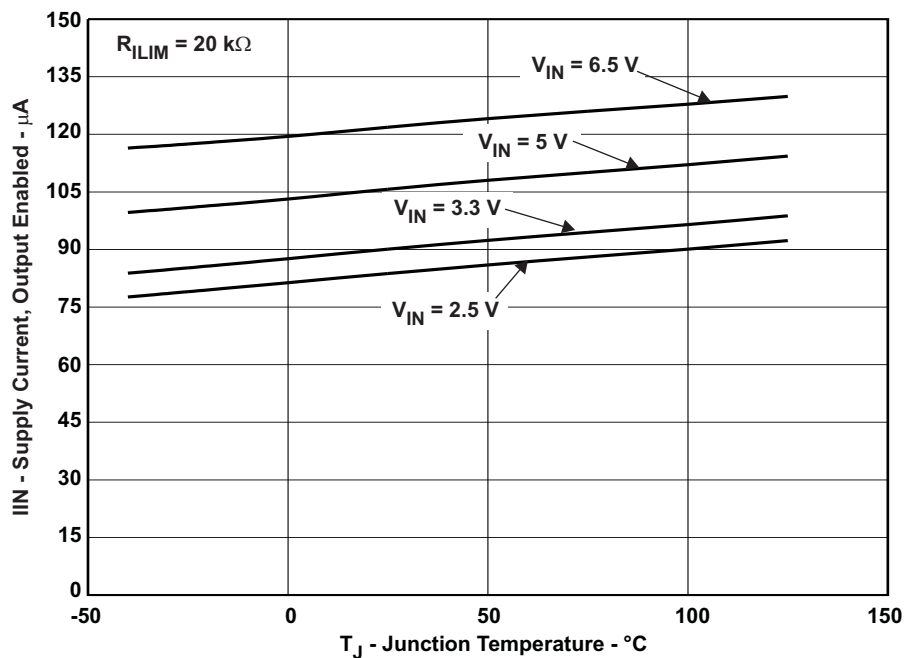
Figure 18. I IN – Supply Current, Output Enabled – μA
