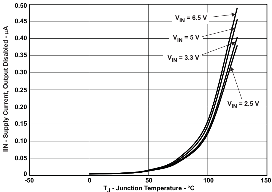
Figure 17. I IN – Supply Current, Output Disabled – μA
