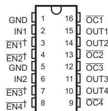
Figure 5-6. TPS2044B and TPS2054B: D Package 16-Pin SOIC Top View
