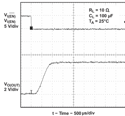
Figure 9-29. Turnon Delay and Rise Time With 100-μF Load
