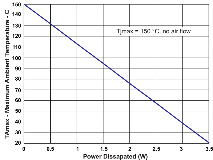
Figure 52. Maximum Ambient Temperature vs IC power Dissipation
