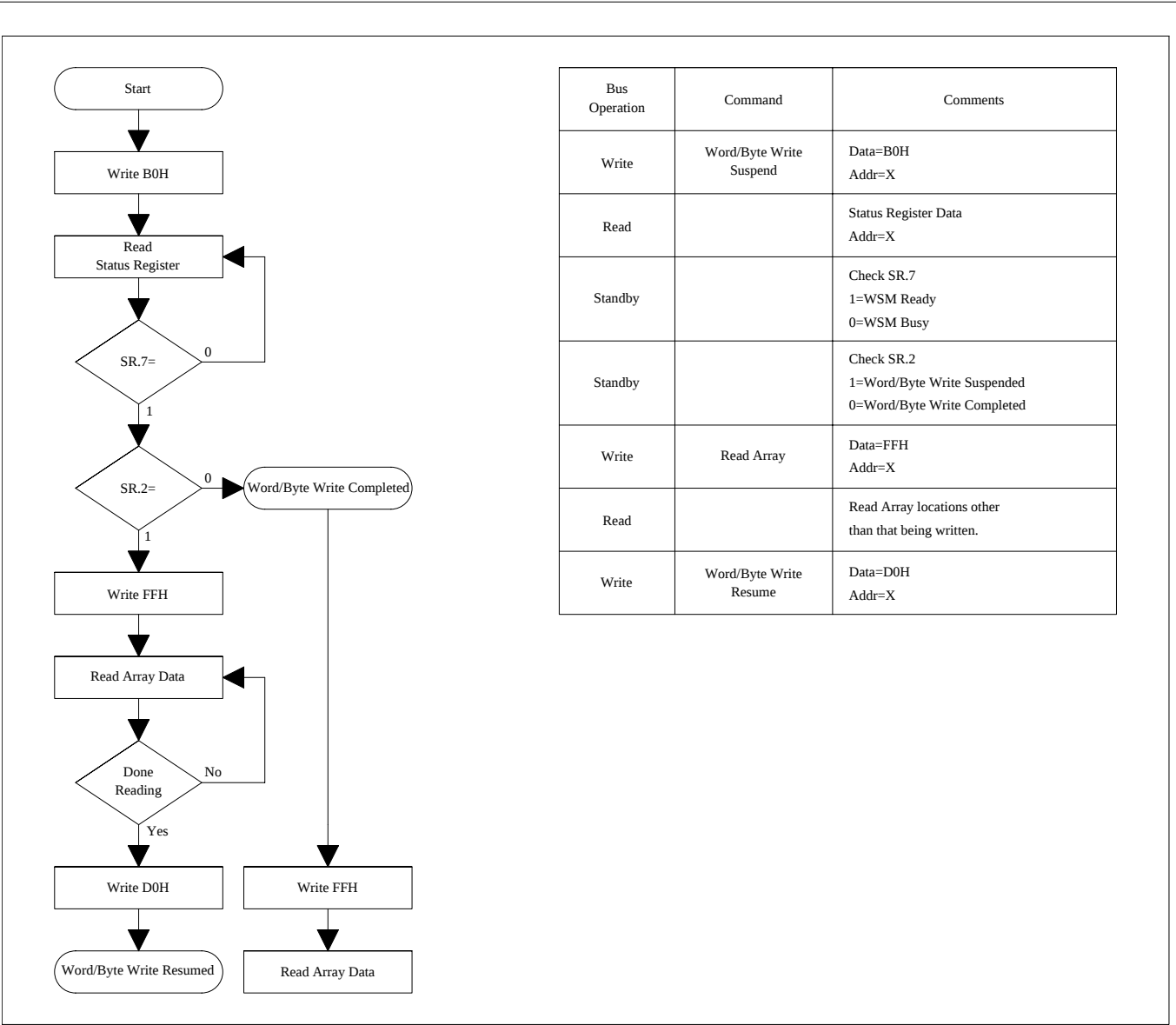
Figure 9. Word/Byte Write Suspend/Resume Flowchart
