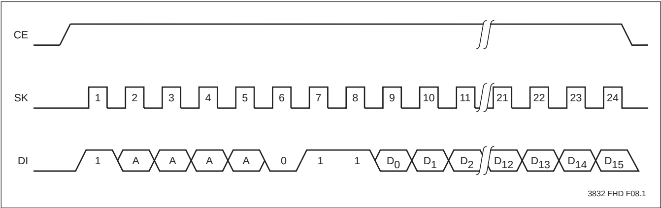
Figure 2. RAM Write
