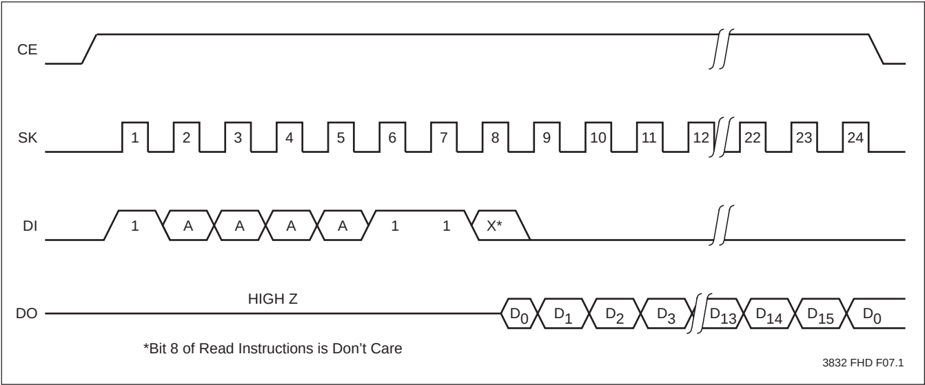
Figure 1. RAM Read
