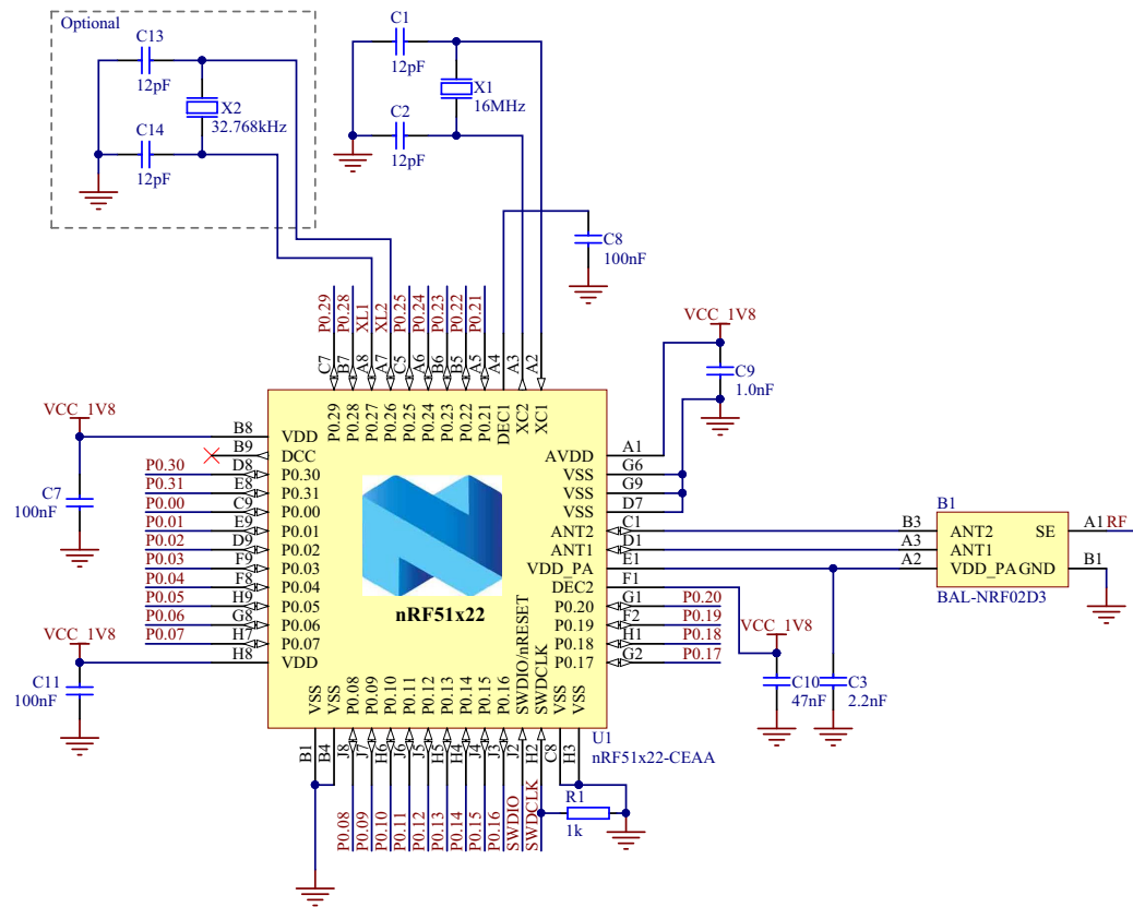
Figure 37 CEAA WLCSP with low voltage mode setup
