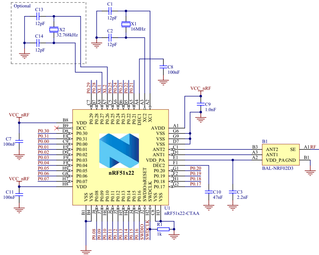
Figure 42 CTAA WLCSP with internal LDO setup
