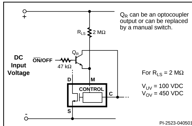
Figure 40. Active-off Remote ON/OFF with LINE-SENSE.
