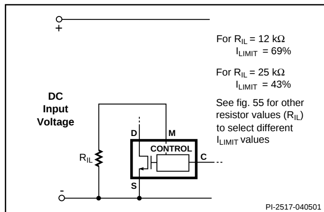
Figure 34. Externally Set Current Limit.
