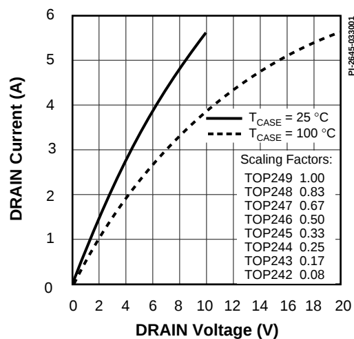
Figure 66. Output Characteristics.
