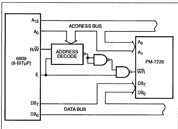
FIGURE 27: PM-7226 to 6809 (8-BIT μP) INTERFACE (Simplified circuit, only lines of interest are shown.)
