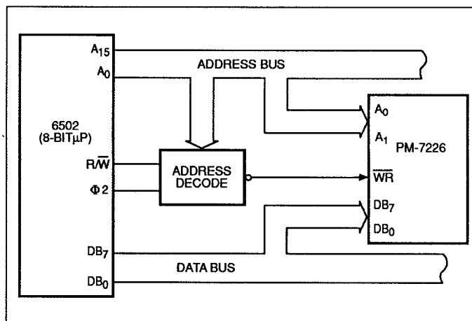
FIGURE 28: PM-7226 to 6502 (8-BIT μP) INTERFACE (Simplified circuit, only lines of interest are shown.)
