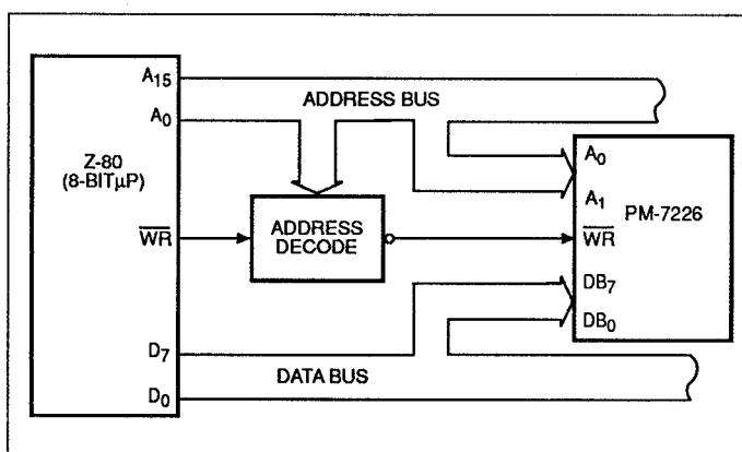
FIGURE 26: PM-7226 to Z-80 (8-BIT μP) INTERFACE (Simplified circuit, only lines of interest are shown.)
