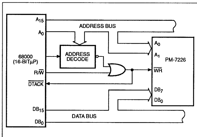
FIGURE 29: PM-7226 to 68000 (16-BIT μP) INTERFACE (Simplified circuit, only lines of interest are shown.)
