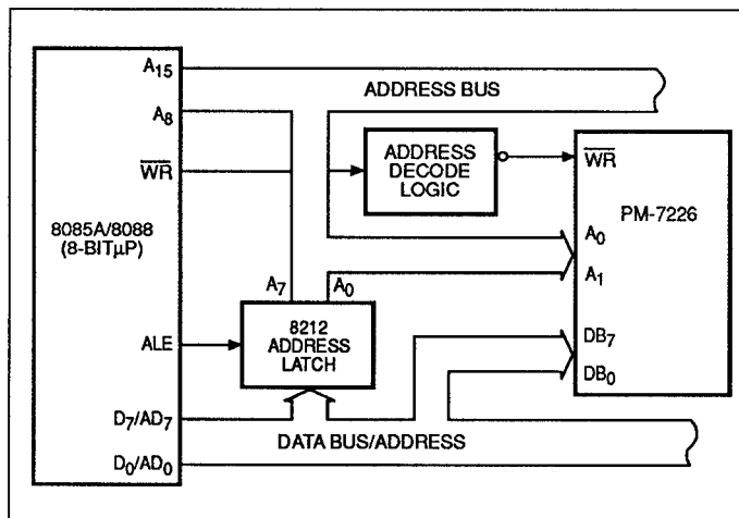
FIGURE 25: PM-7226 to 8085A/8088 (8-BIT μP) INTERFACE (Simplified circuit, only lines of interest are shown.)
