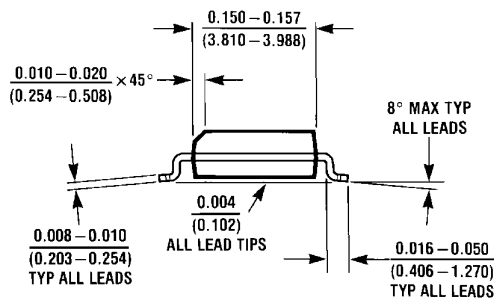
SO-8 Package NS Package Number M08A
