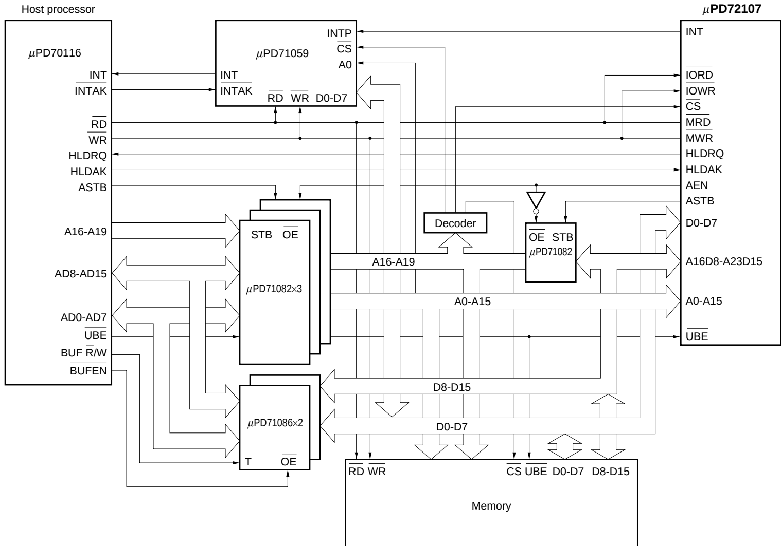
μPD72107 System Configuration Example (Main Memory Sharing Type)
