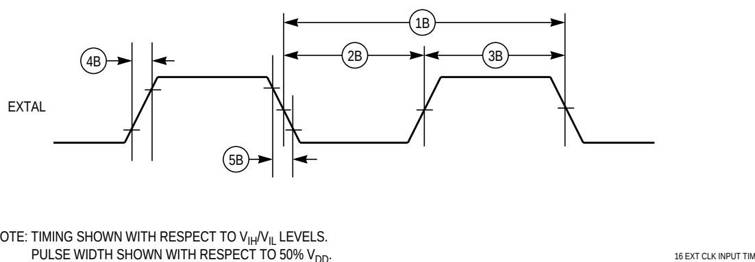
Figure A-2 External Clock Input Timing Diagram
