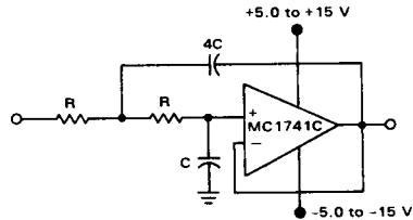
FIGURE 20 — OPERATIONAL AMPLIFIER LOW PASS FILTER
