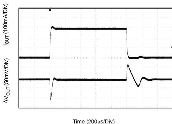
Figure 22. Load Transient Response (Conditions: V_{IN}=2.5V , V_{OUT}=1.3V , I_{OUT}=1mA to 300mA , C_{IN}=1\mu F , C_{OUT}=2.2\mu F )
