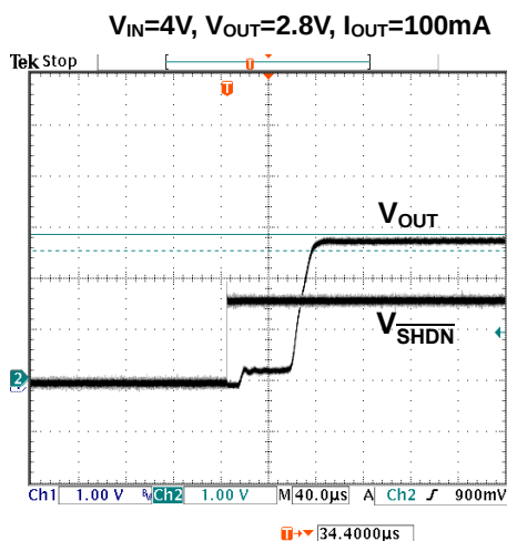
Figure 14. Shutdown/Enable Test
