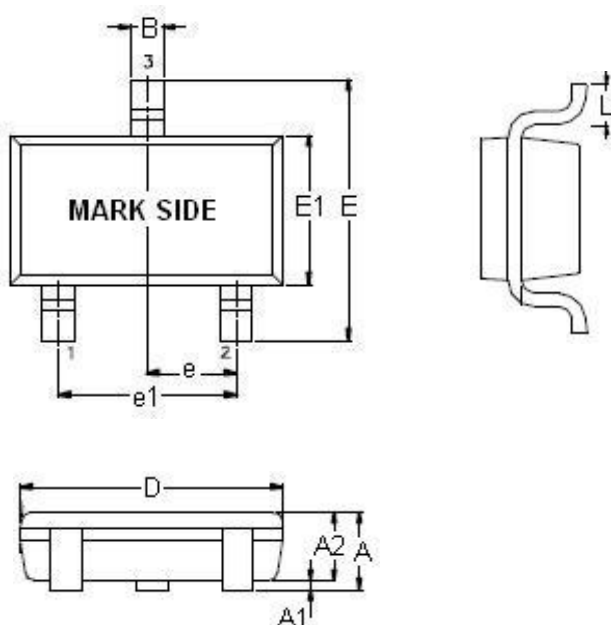
SOT-23-3 Package (Unit: mm)
