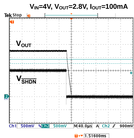
Figure 15. Shutdown/Enable Test
