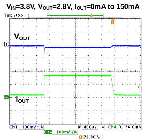
Figure 13. Load Transition Response
