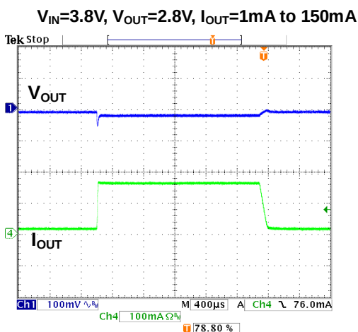
Figure 12. Load Transition Response
