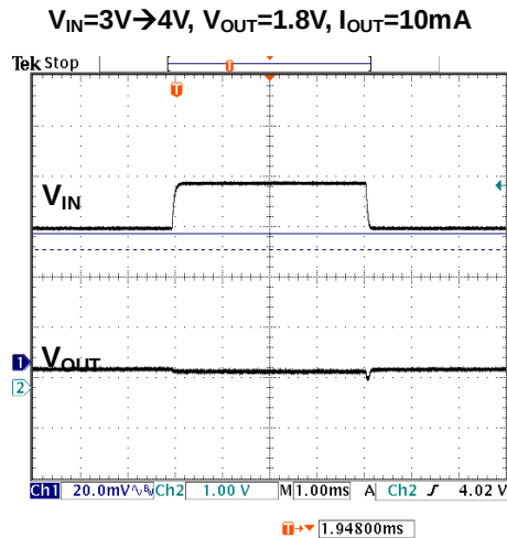
Figure 16. Line Transition Response
