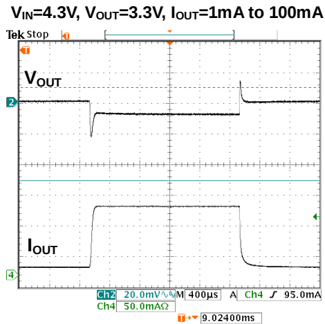
Figure 10. Load Transition Response
