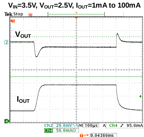
Figure 11. Load Transition Response
