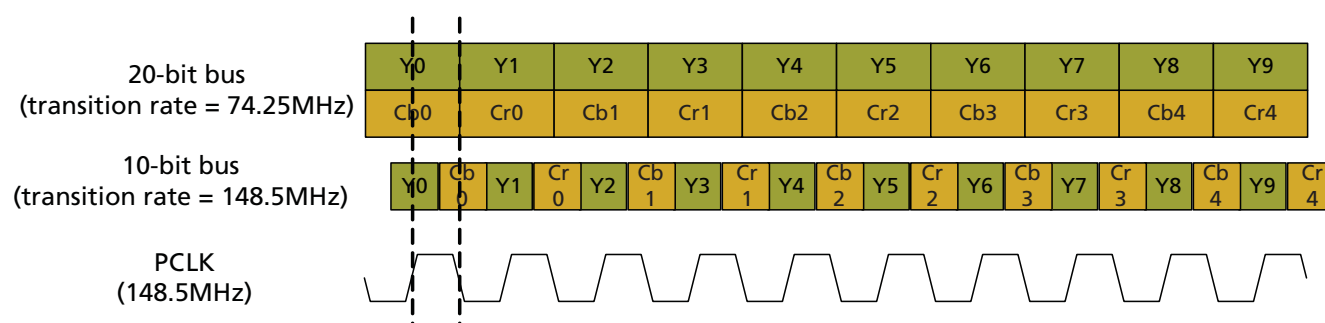
Figure 4-7: DDR Video Interface
