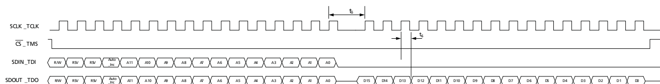
Figure 4-37: Read Mode
