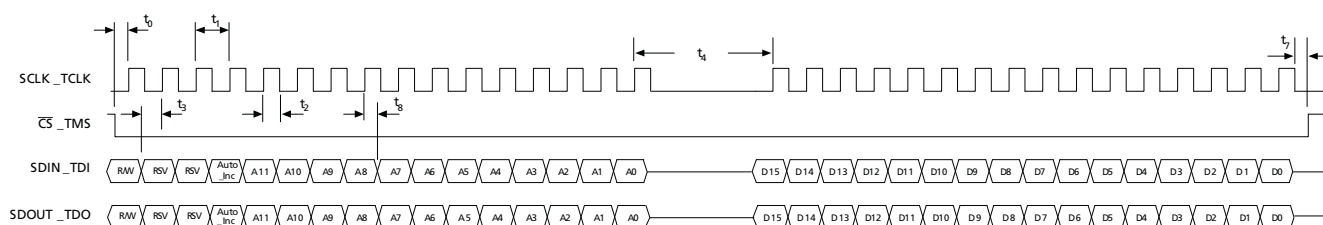
Figure 4-36: Write Mode
