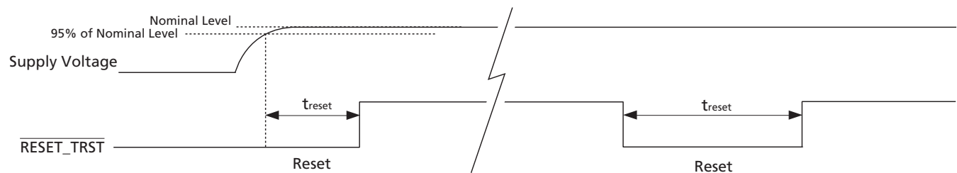
Figure 4-41: Reset Pulse
