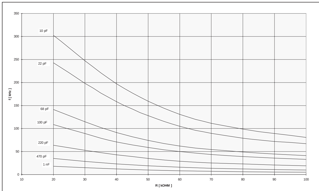
Figure 9 Switching Frequency
