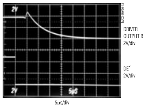
MAX1480B DRIVER DISABLE TIME
