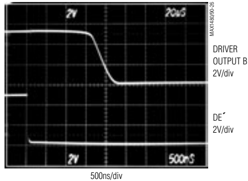
MAX1480C DRIVER DISABLE TIME
