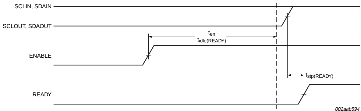
Fig 18. t_{stp(READY)} delay that can occur after t_{en} and t_{idle(READY)}
