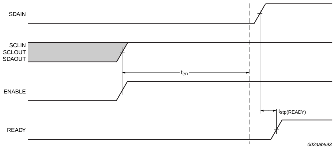
Fig 17. t_{stp(READY)} that can occur after t_{en}
