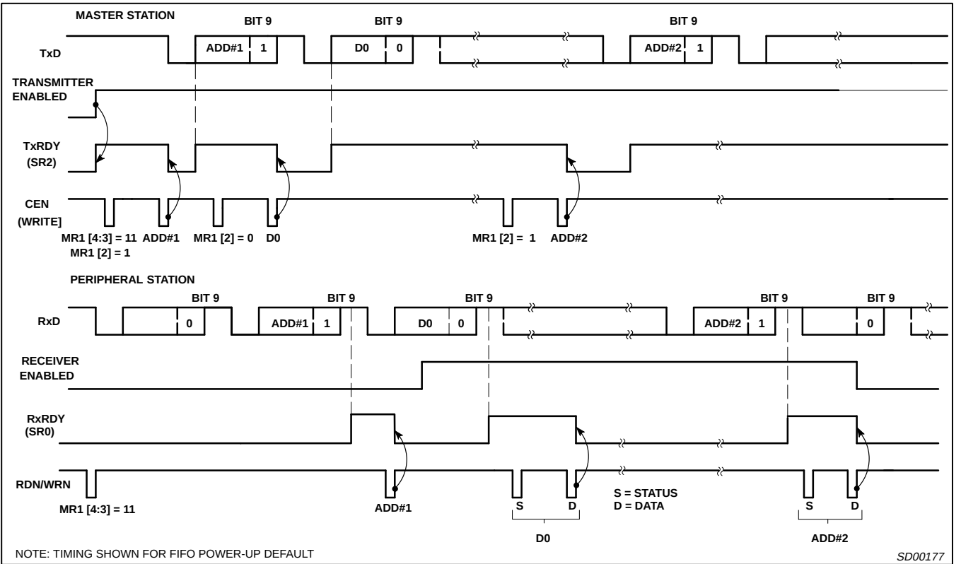
Figure 15. Wake-Up Mode
