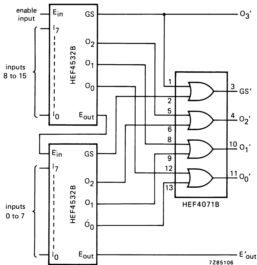
Fig.5 16-level priority encoder.
