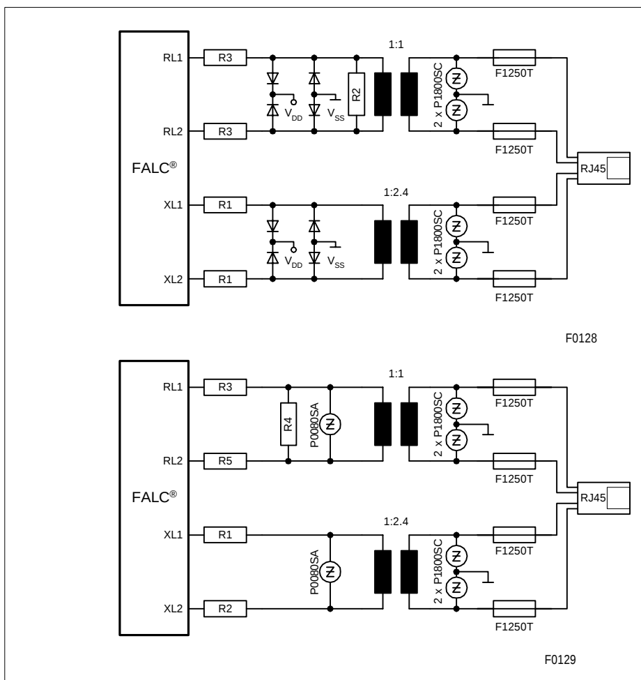
Figure 83 Protection Circuitry
