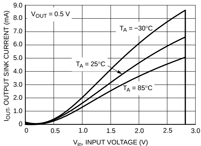
Figure 28. NCP302H/3L Series 2.7 V Reset Output Sink Current vs. Input Voltage
