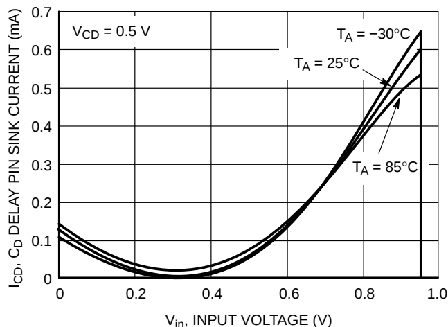
Figure 30. NCP302/3 Series 0.9 V C_D Delay Pin Sink Current vs. Input Voltage
