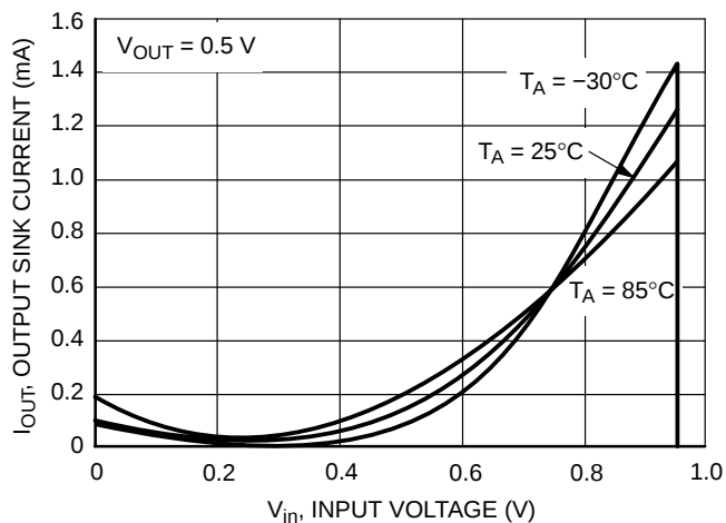
Figure 27. NCP302H/3L Series 0.9 V Reset Output Sink Current vs. Input Voltage
