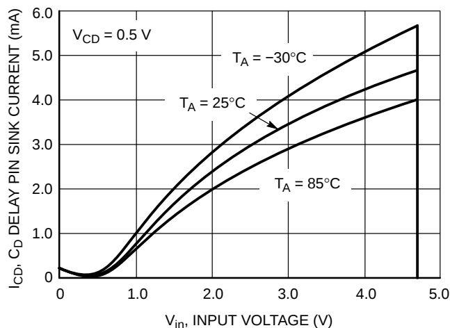
Figure 32. NCP302/3 Series 4.5 V C_D Delay Pin Sink Current vs. Input Voltage
