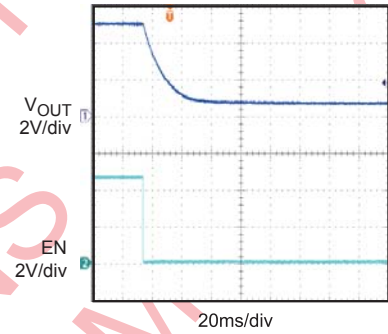
Turn Off Delay and Fall Time with 10uF Load Cout=10uF, no load
