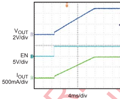
Turn On Delay and Rise Time with 10uF Load Rload=5Ω
