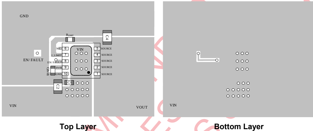
Figure 3—PCB Layout
