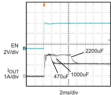
Inrush Current with Different Load Capacitance Rload=3.9Ω, no Cdv/dt, EN Floating
