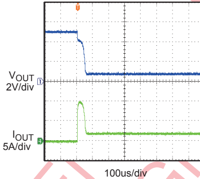
0.33 \Omega Load Connected to Enabled Device
