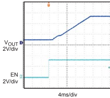
Turn On Delay and Rise Time with 1uF Load, 1nF Cdv/dt Cout=1uF, no load
