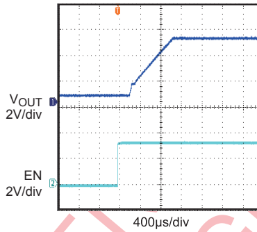
Turn On Delay and Rise Time with 1uF Load, no Cdv/dt Cout=1uF, no load
