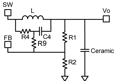
Figure 9—Simplified Circuit of Ceramic Capacitor
