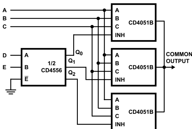
Figure 6-17. 24-to-1MUX Addressing
