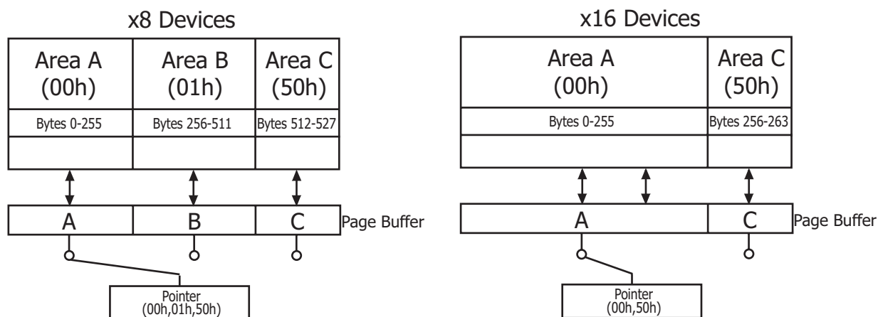
Figure 29: Pointer operations
