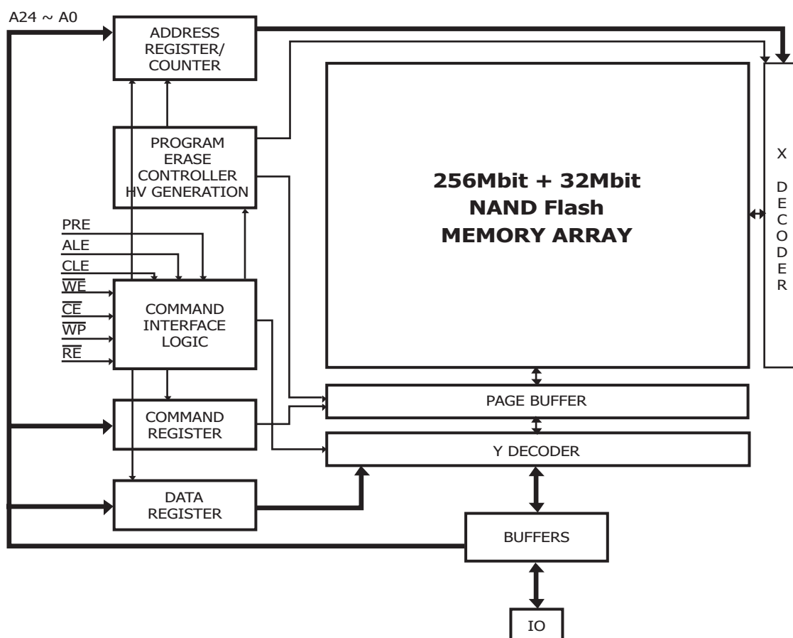
Figure 6: Block Diagram
