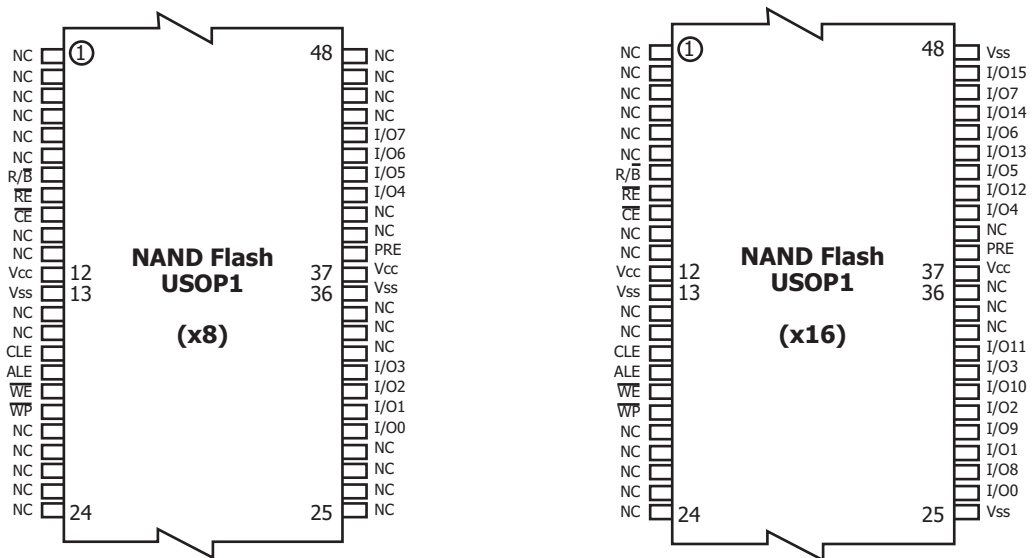
Figure 3. 48USOP1 Contactations, x8 and x16 Device
