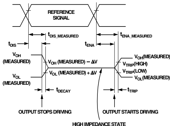
Figure 41. Output Enable/Disable
