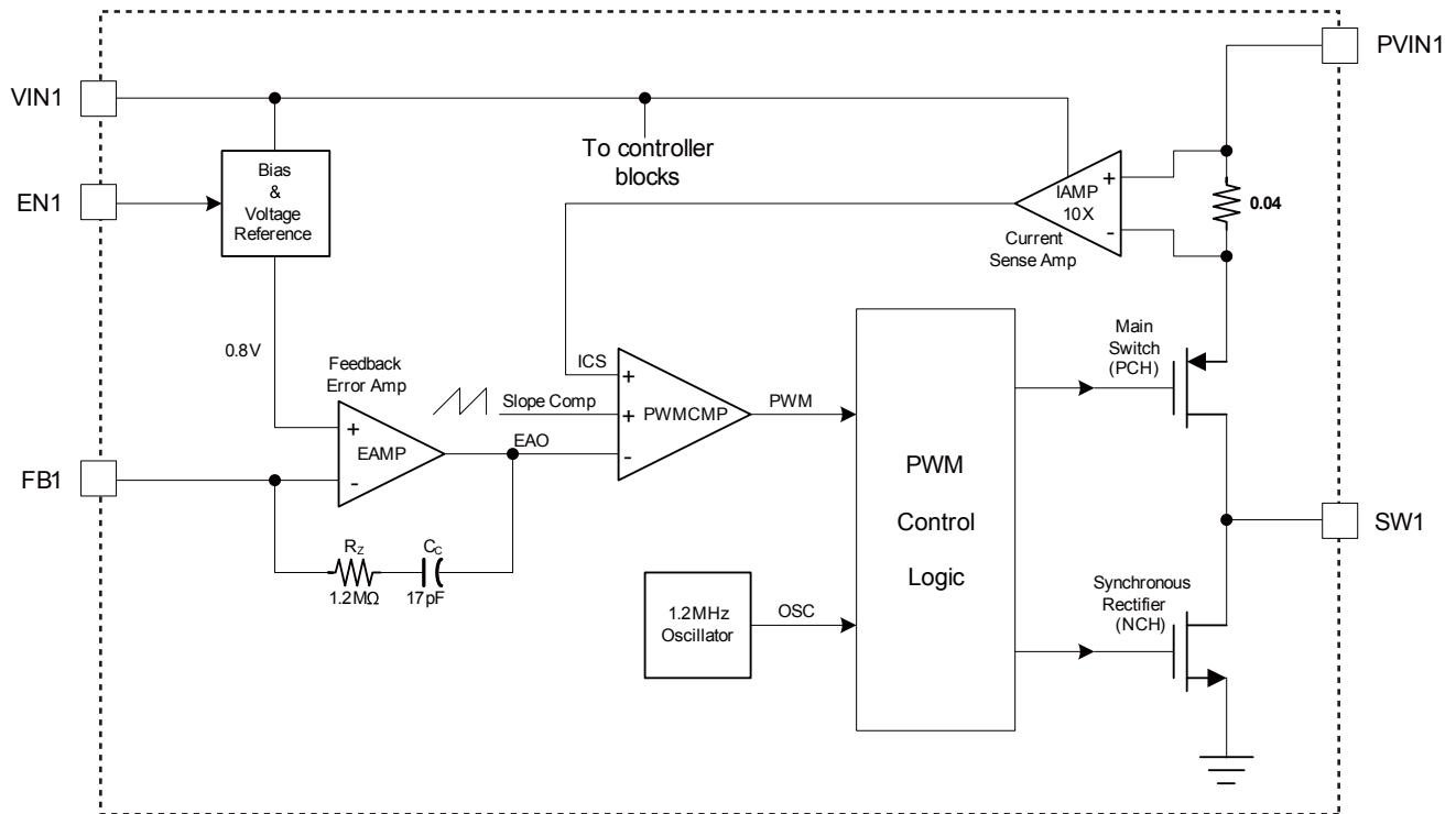
Figure 1 -Functional Block Diagram (1/2 of the MP2125)
