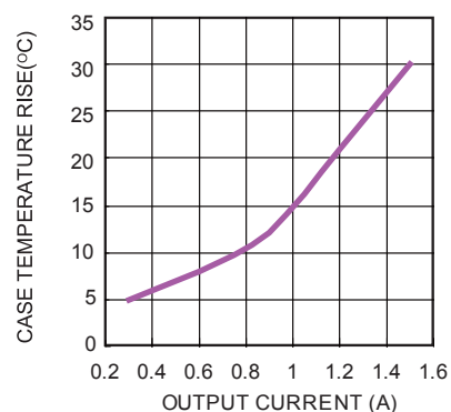
Case Temperature Rises vs. Output Current
