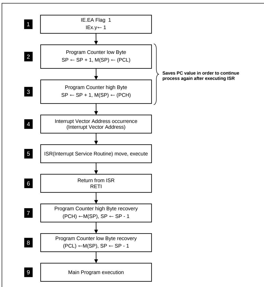
Figure 10-4 Interrupt Execution Sequence
