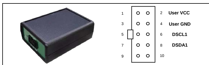
Figure 1-2 On Chip Debugger 2 and Pin description (ocd2 mode 1)
