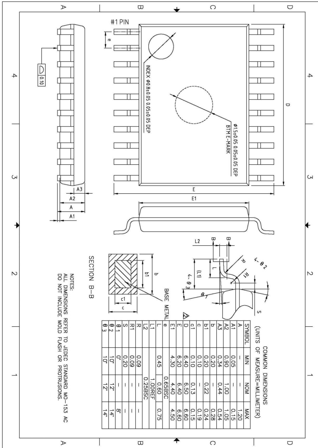
Figure 4-3 20 pin TSSOP package
