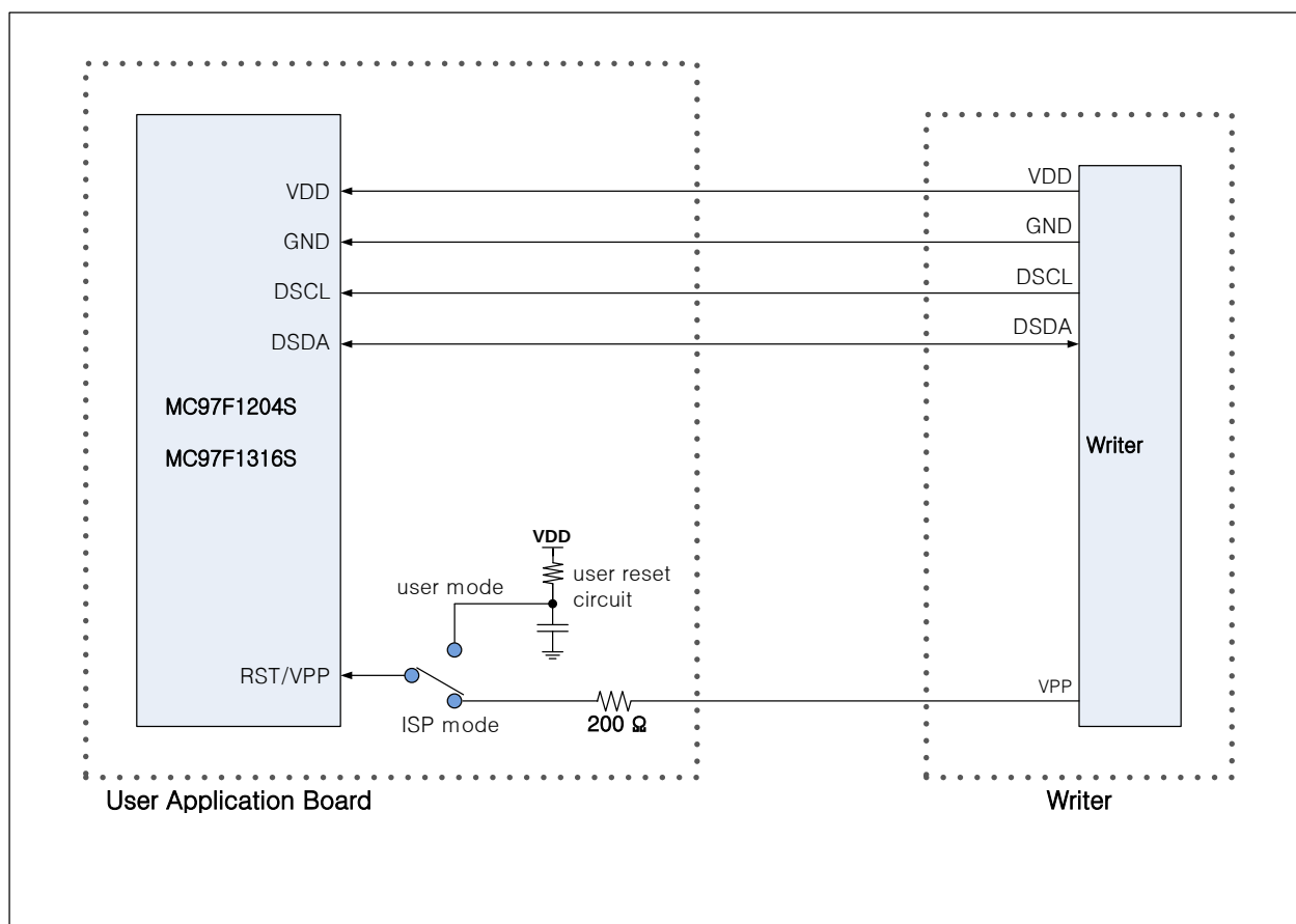
Figure 1-6 ISP Interface
