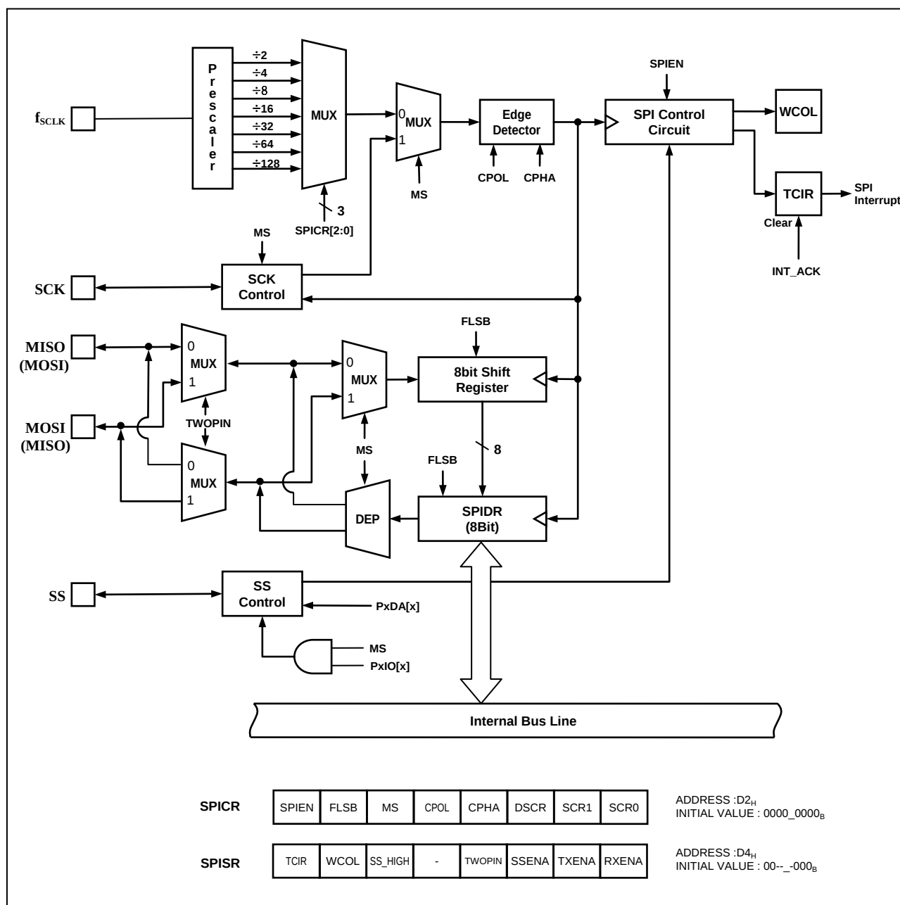
Figure 11-10 SPI Block Diagram
