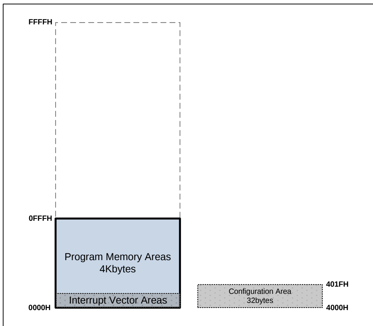
Figure 8-1 Program Memory
