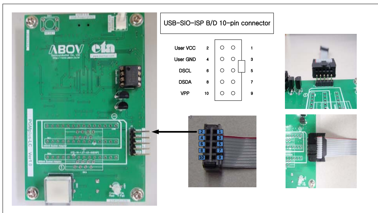
Figure 1-4 PGMplusLC Writer
