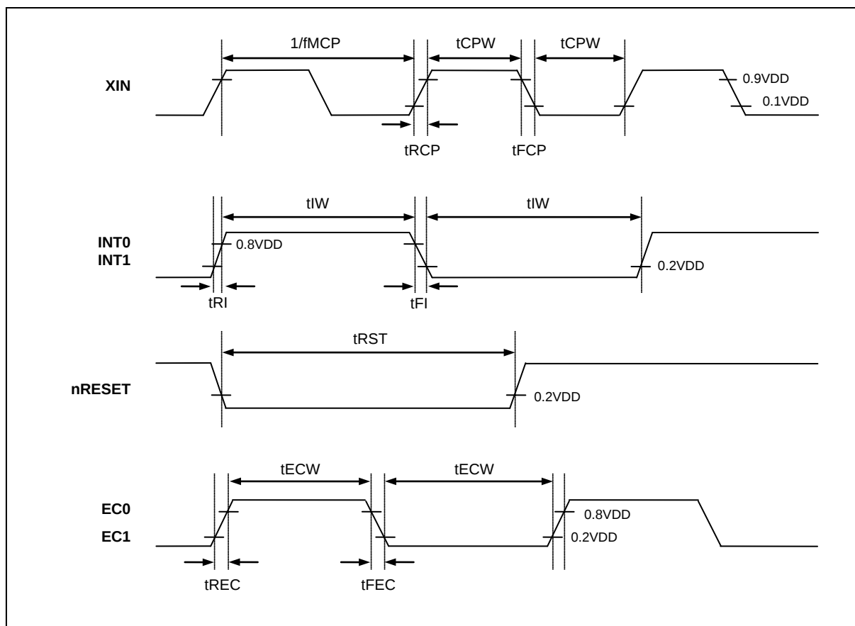
Figure 7-1 AC Timing
