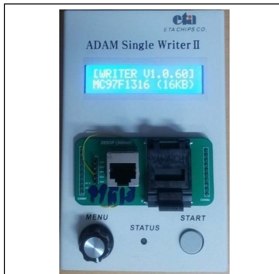
Figure 1-3 Single Programmer
