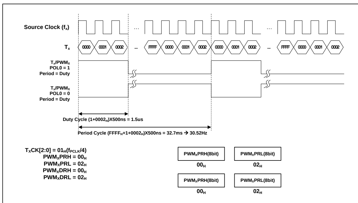
Figure 11-9 Example of PWM at 8MHz (Period = Duty)
