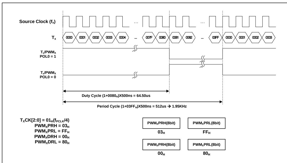
Figure 11-8 Example of PWM at 8MHz
