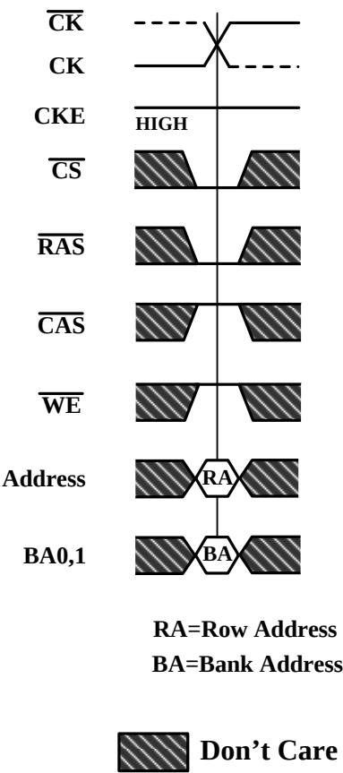
Figure 5. tRCD and tRRD Definition
