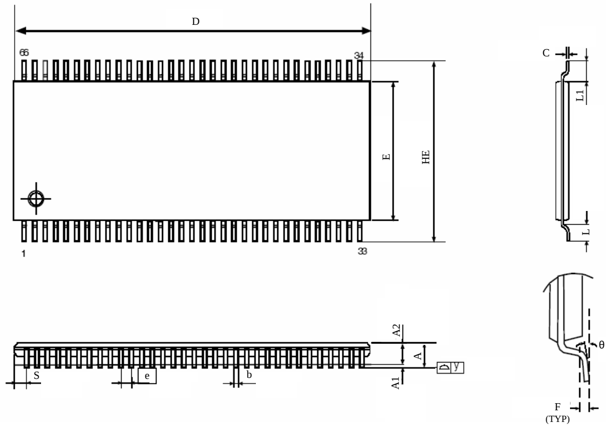
Figure 43. 66 Pin TSOP II Package Outline Drawing Information
