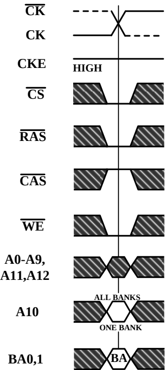
Figure 27. Precharge Command
