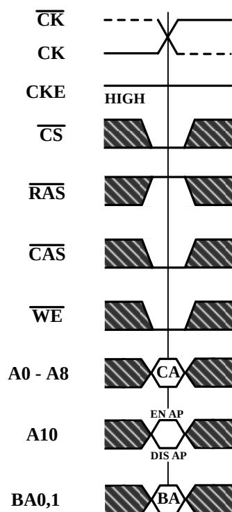
Figure 14. Write Command
