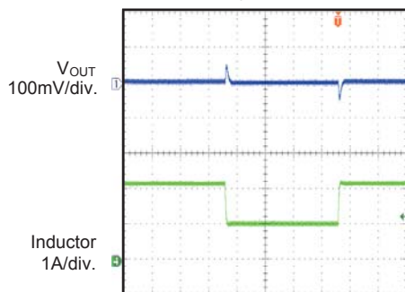
Load Transient
