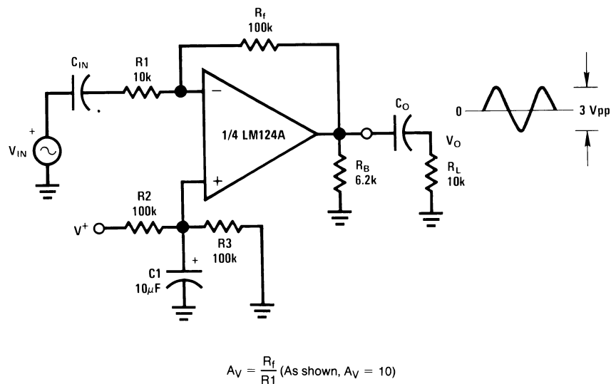
Figure 37. AC Coupled Inverting Amplifier
