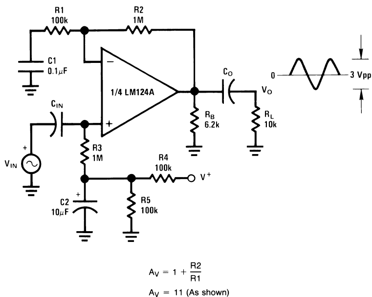
Figure 38. AC Coupled Non-Inverting Amplifier
