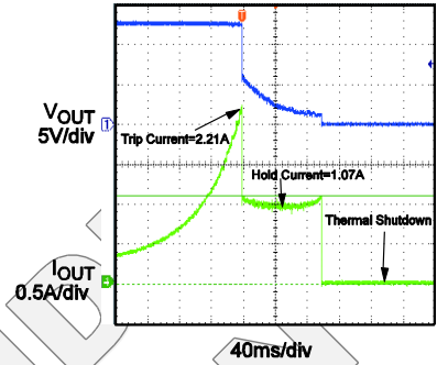
Current Limit R_{LIMIT}=100\Omega
