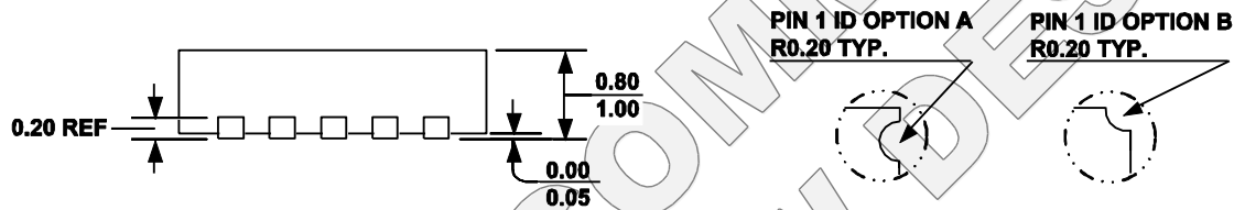
SIDE VIEW
