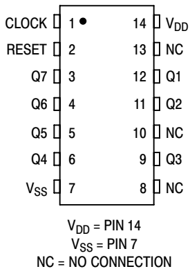
PIN ASSIGNMENT
