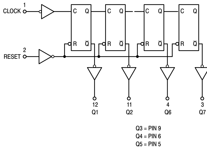
LOGIC DIAGRAM
