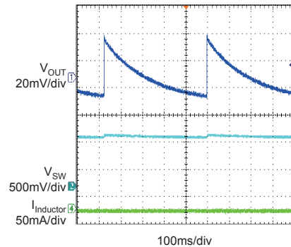
Output Ripple Voltage for ASYN Mode
