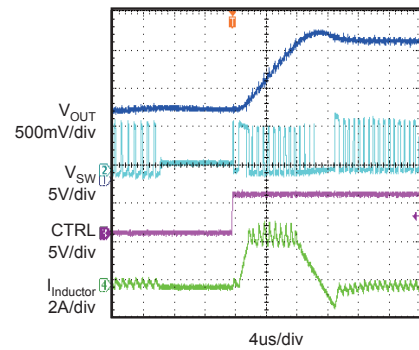
ASYN Mode to PWM Mode
