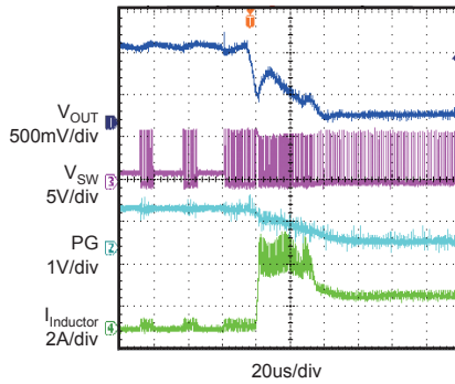
Output Short for ASYN Mode
