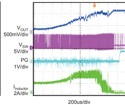
Short Recovery for ASYN Mode
